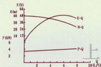
ZW50-20-35
